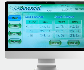
THDi compensation performance
