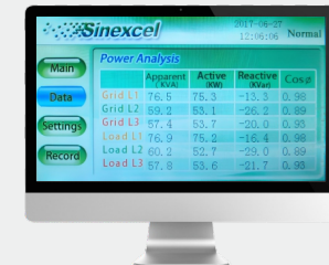
PF compensation performance
