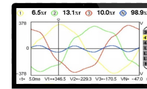
Before THDu governance
